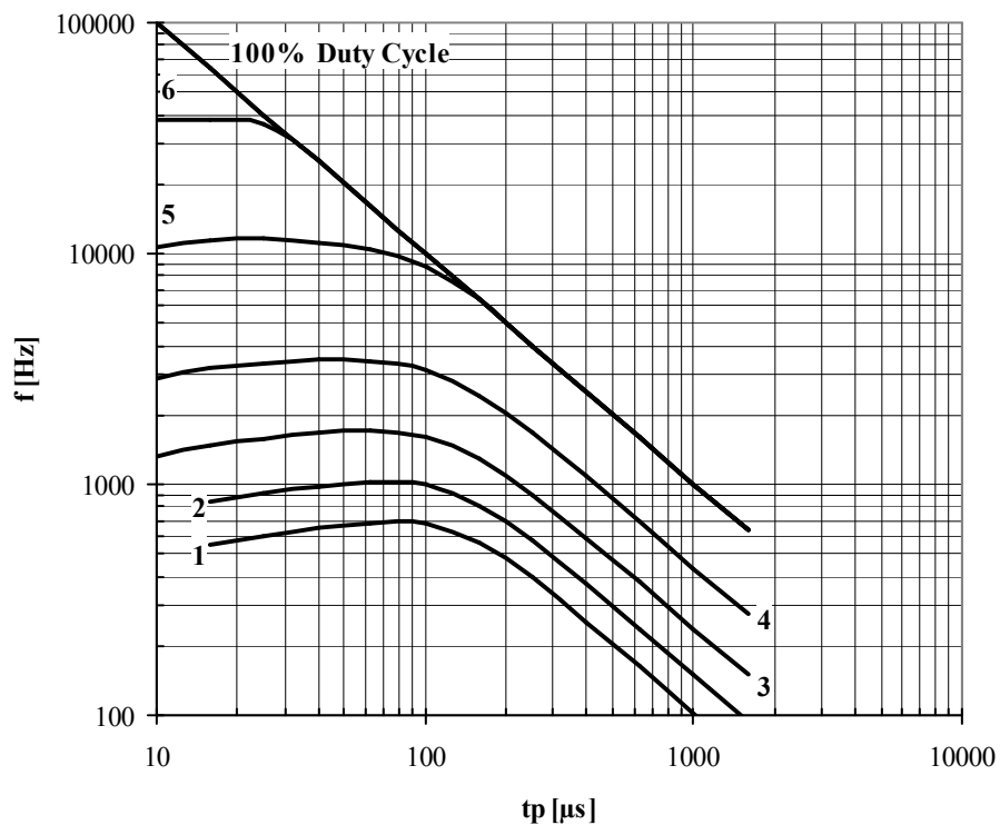
Fig. 11 Sine wave frequency ratings
