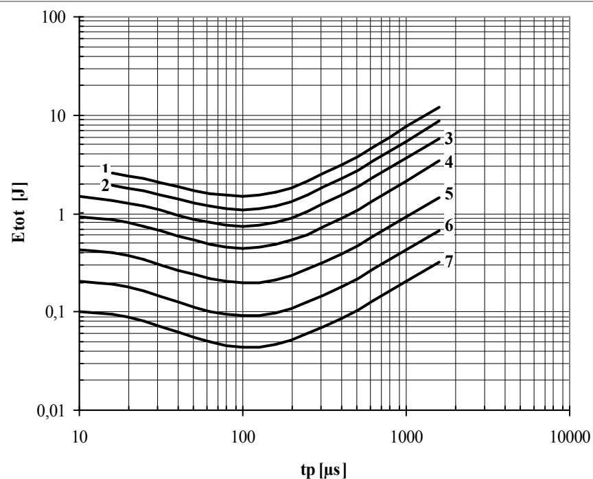
Fig. 23 Sine wave loss energy per pulse
