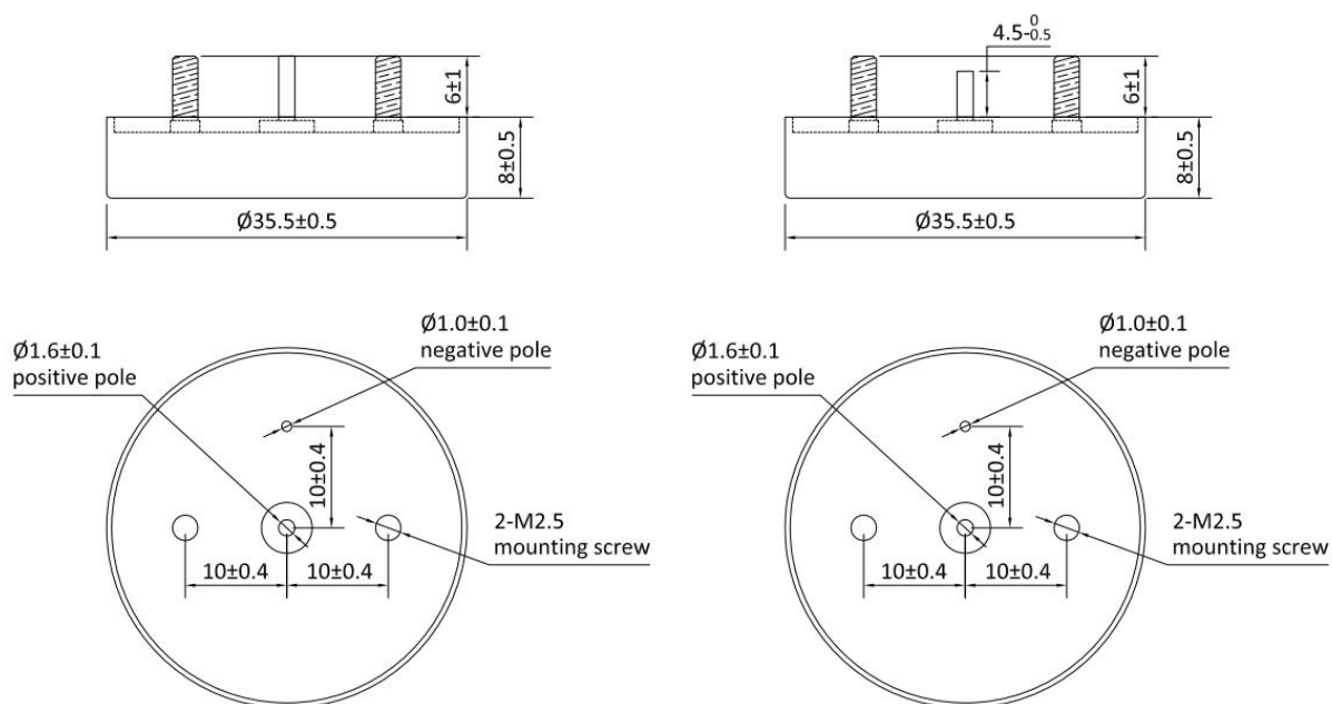
THC1W Ø35.5X8 Layout(A type)
